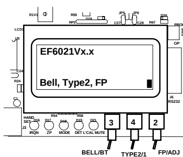
Figure 2 Function Selection
