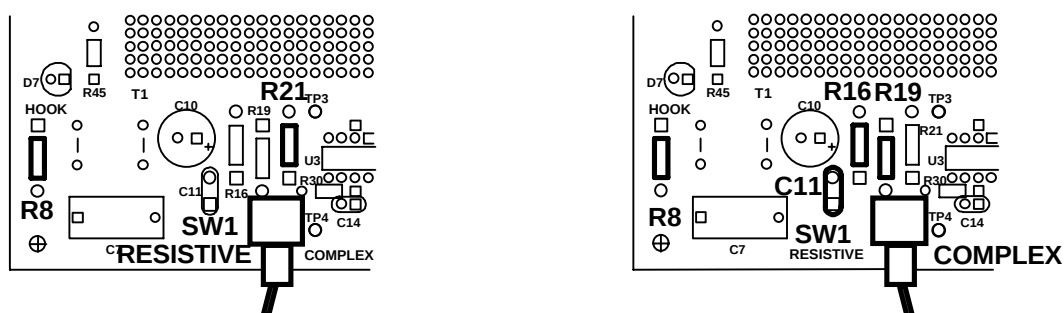
Figure 3 Termination Positions
