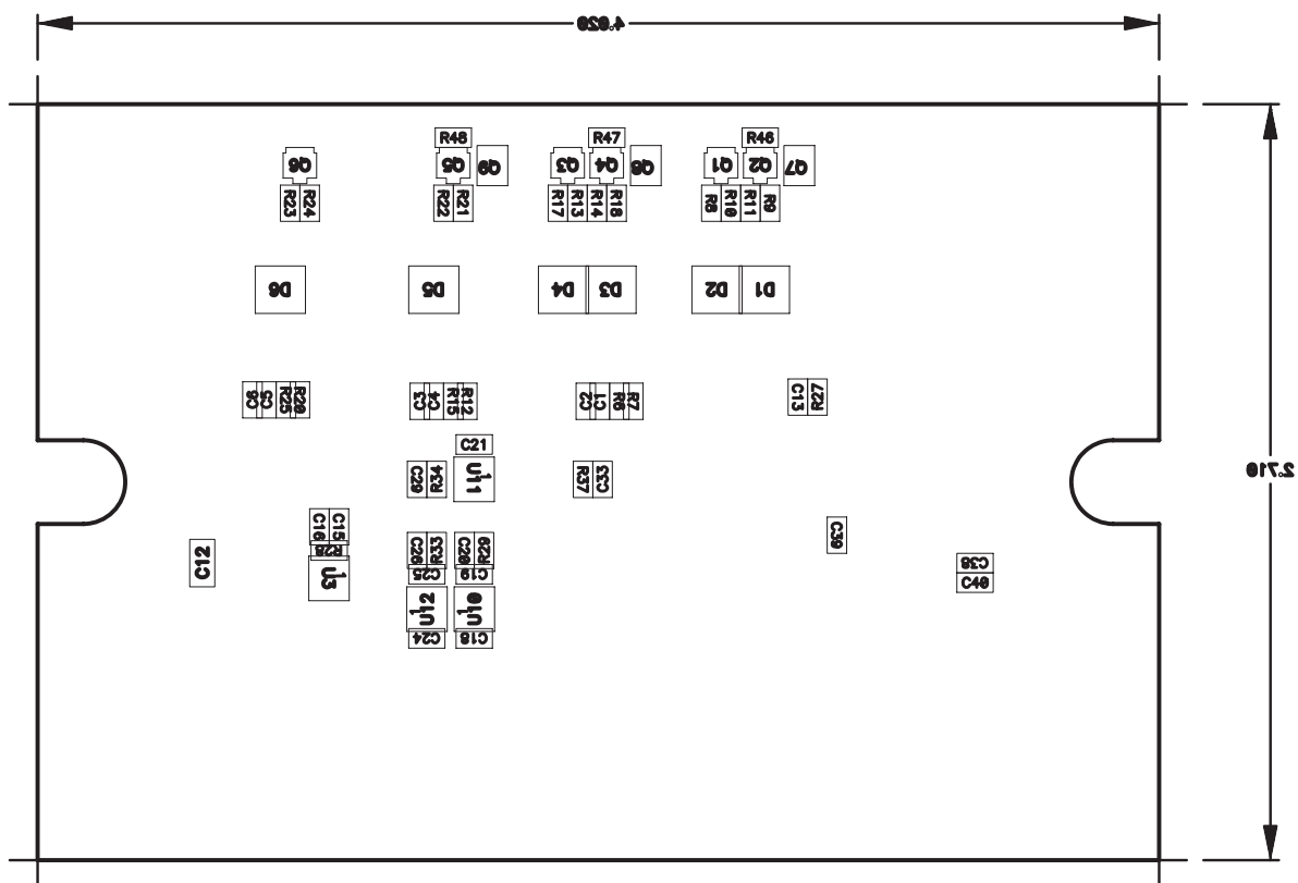
Figure 5. Bottom Assembly
