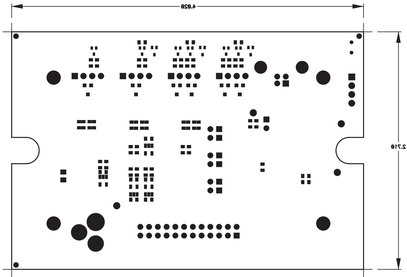
Figure 9. Solder Mask 2
