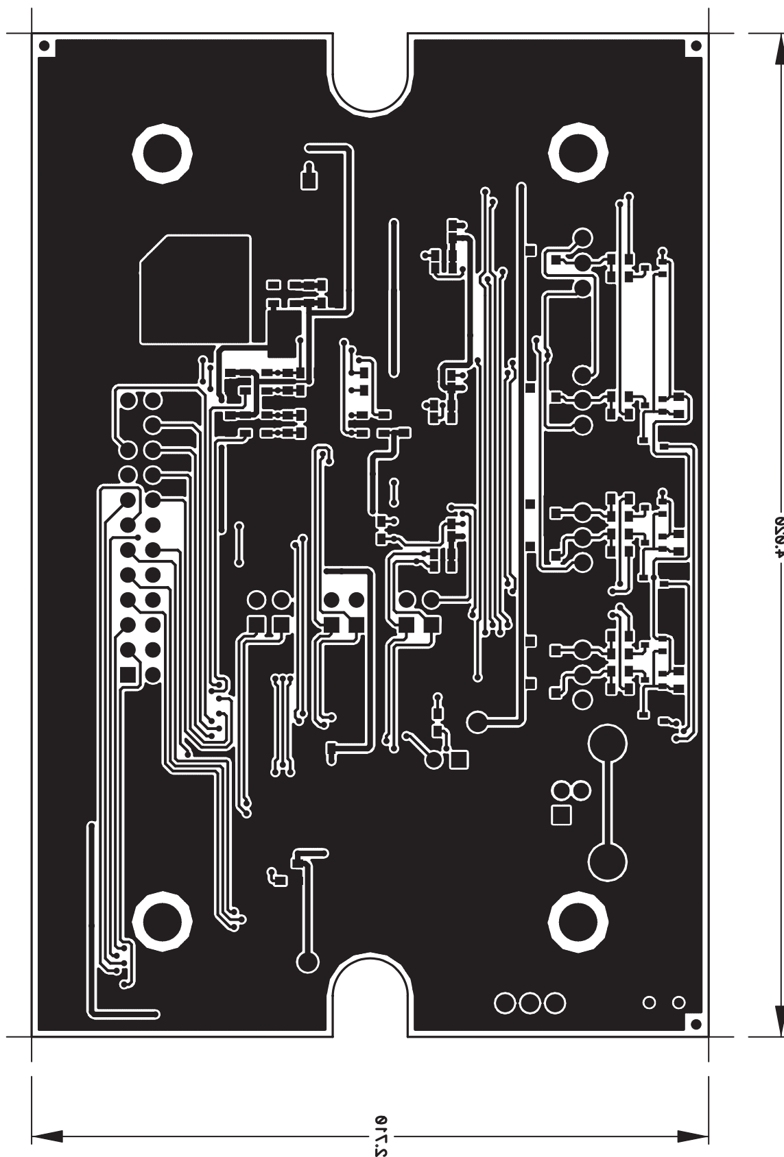
Figure 7. Board Layer 2
