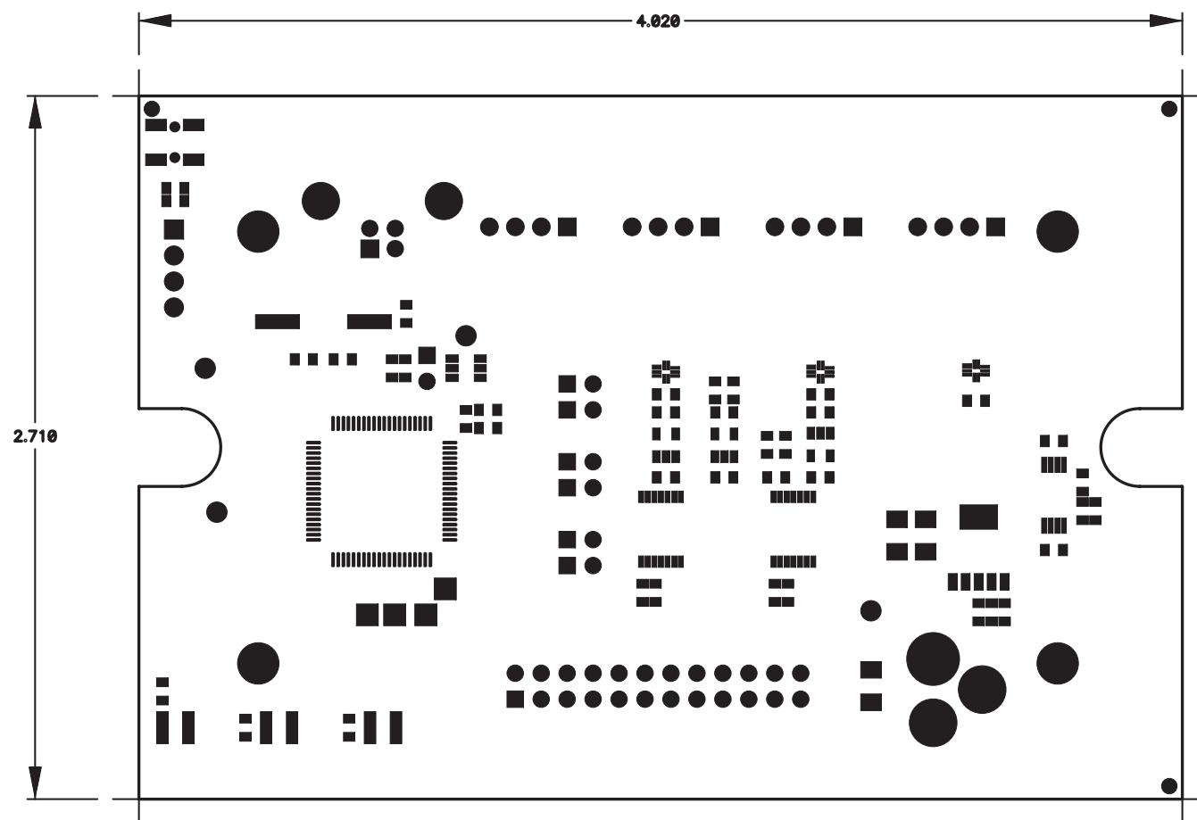
Figure 8. Solder Mask 1
