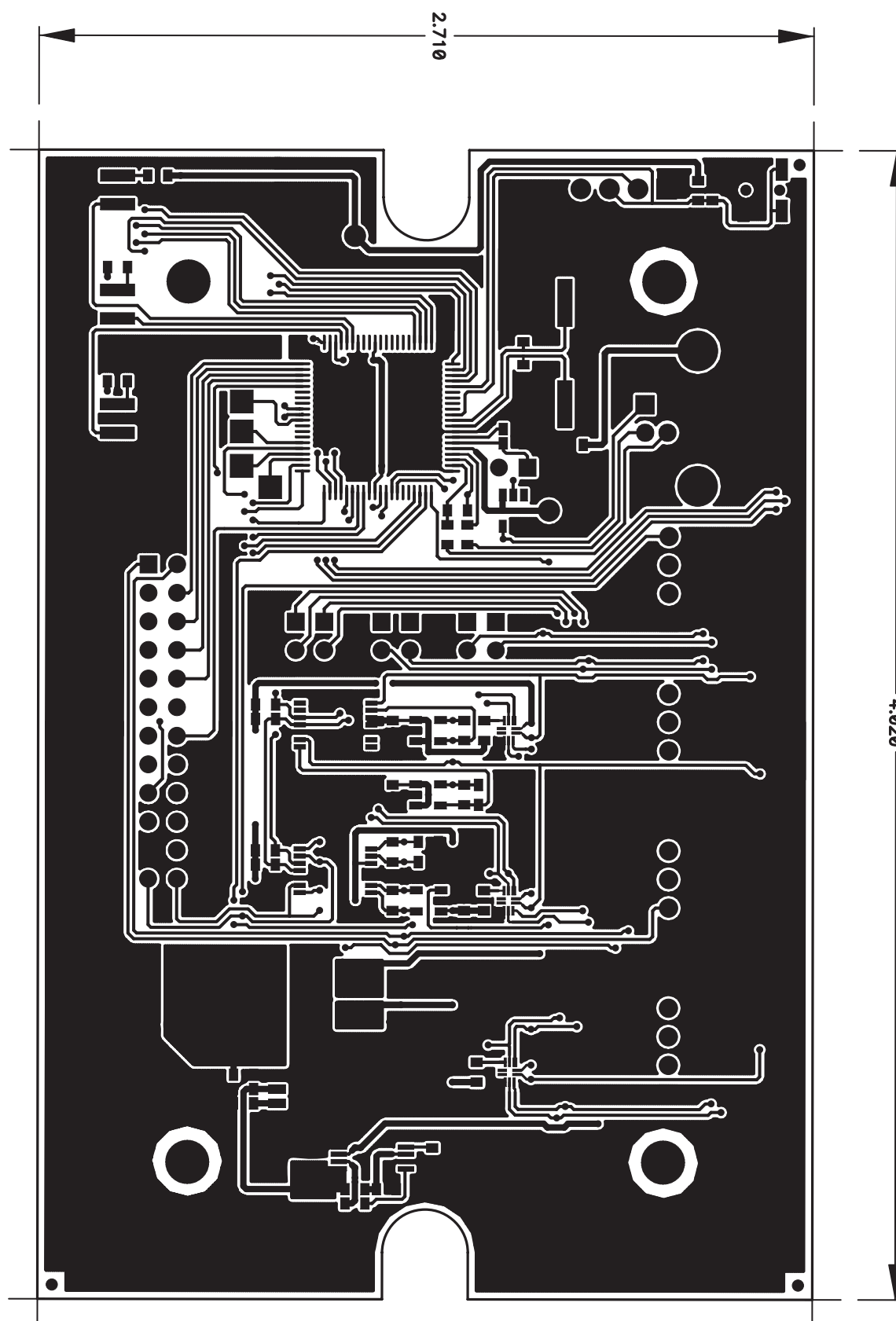
Figure 6. Board Layer 1
