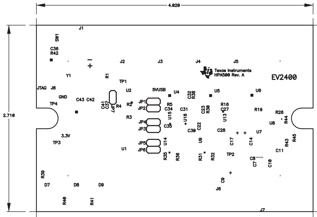
Figure 10. Silkscreen
