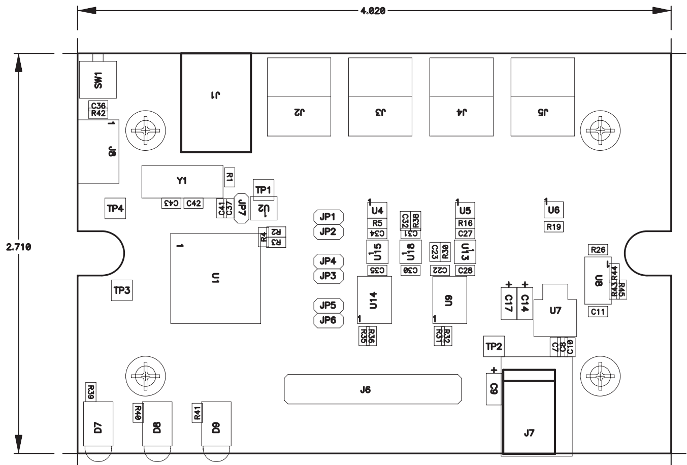
Figure 4. Top Assembly
