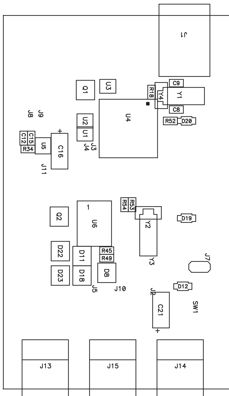
Figure 5. Component Placement 1
