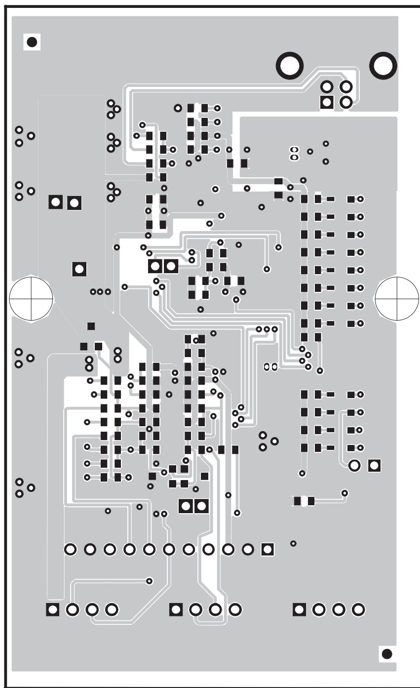
Figure 4. Board Layer 2
