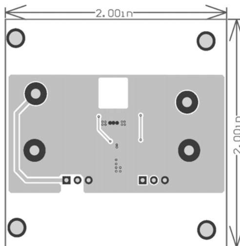
Figure 3: Bottom Silkscreen Layer
