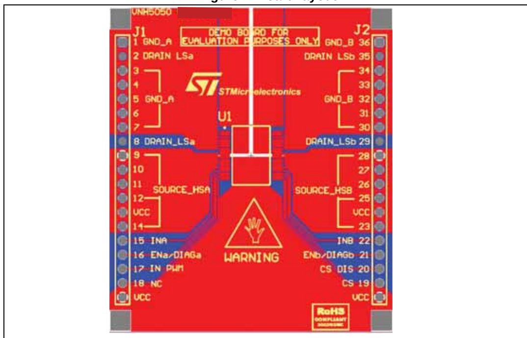
Figure 2. Board layout
