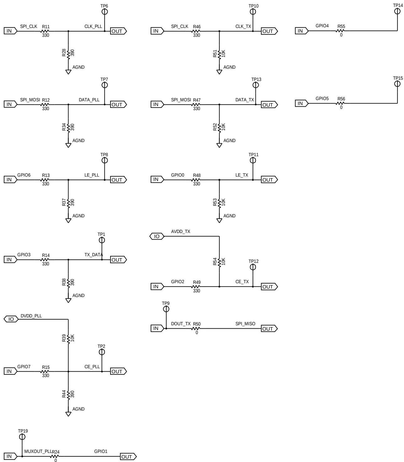
Figure 13. EV-ADF5901SD2Z Schematic (Page 7)
