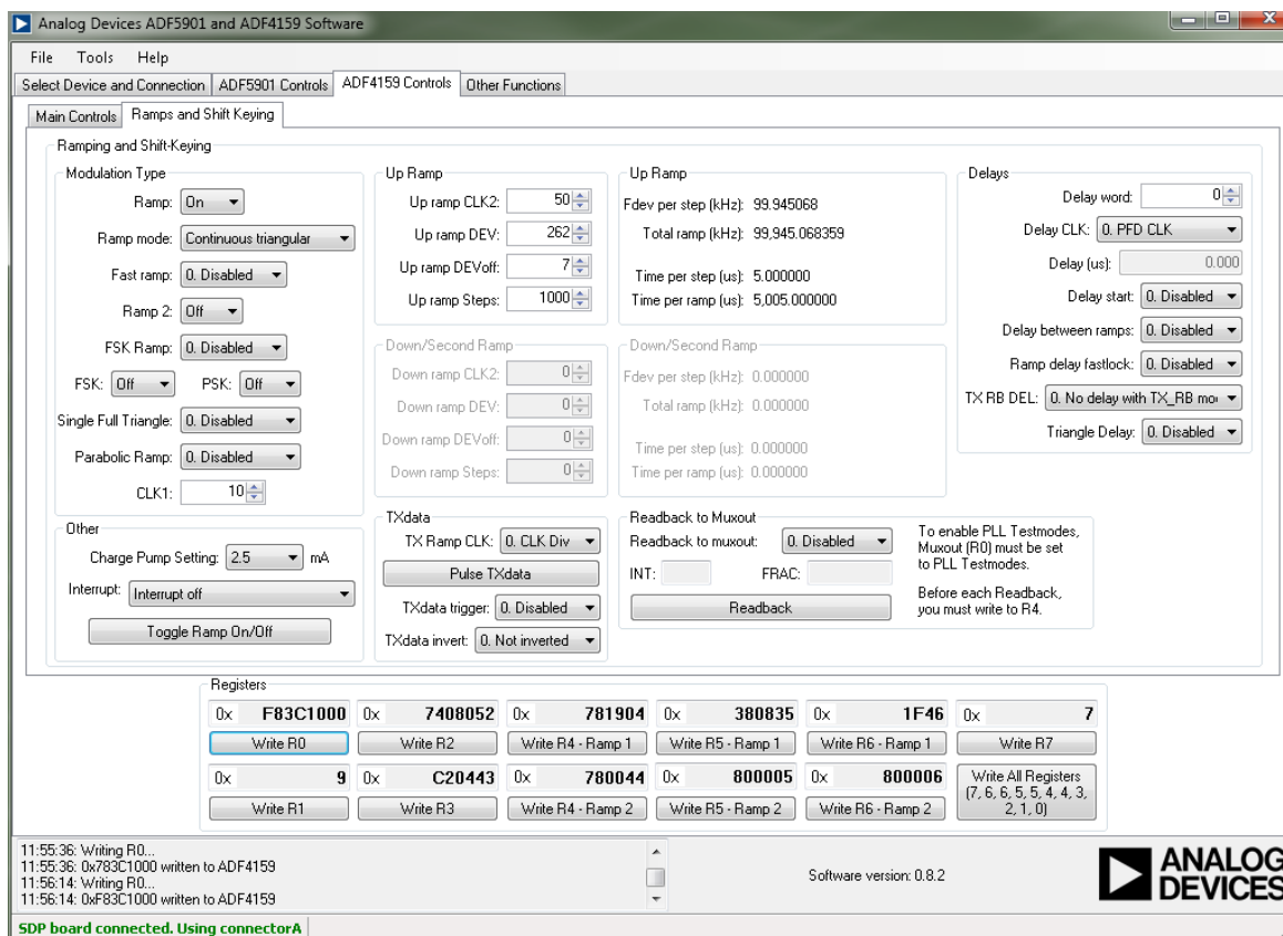
Figure 5. Software Front Panel Display— ADF4159 Ramps and Shift Keying
