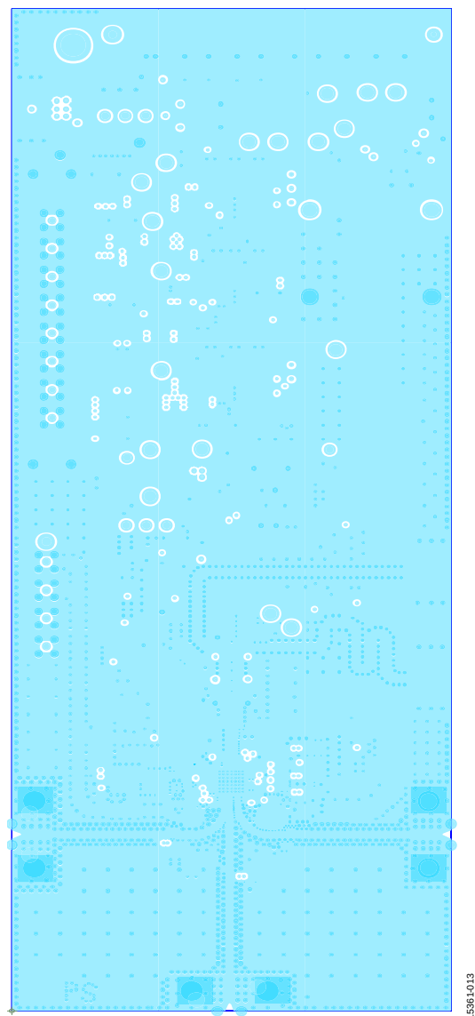
Figure 13. Evaluation Board Layer 2—Ground
