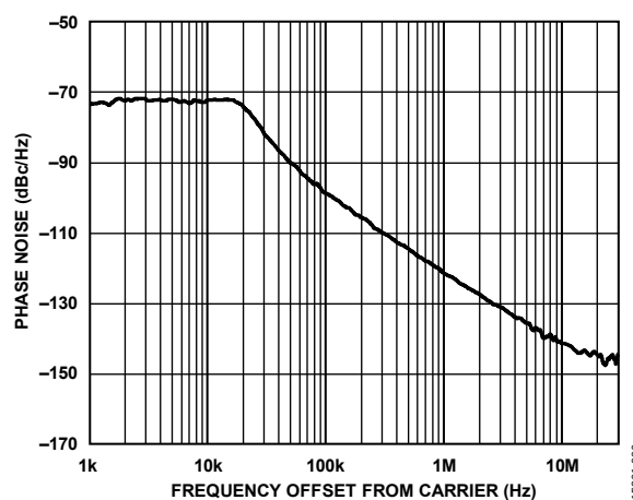
Figure 6. Single Sideband Phase Noise
