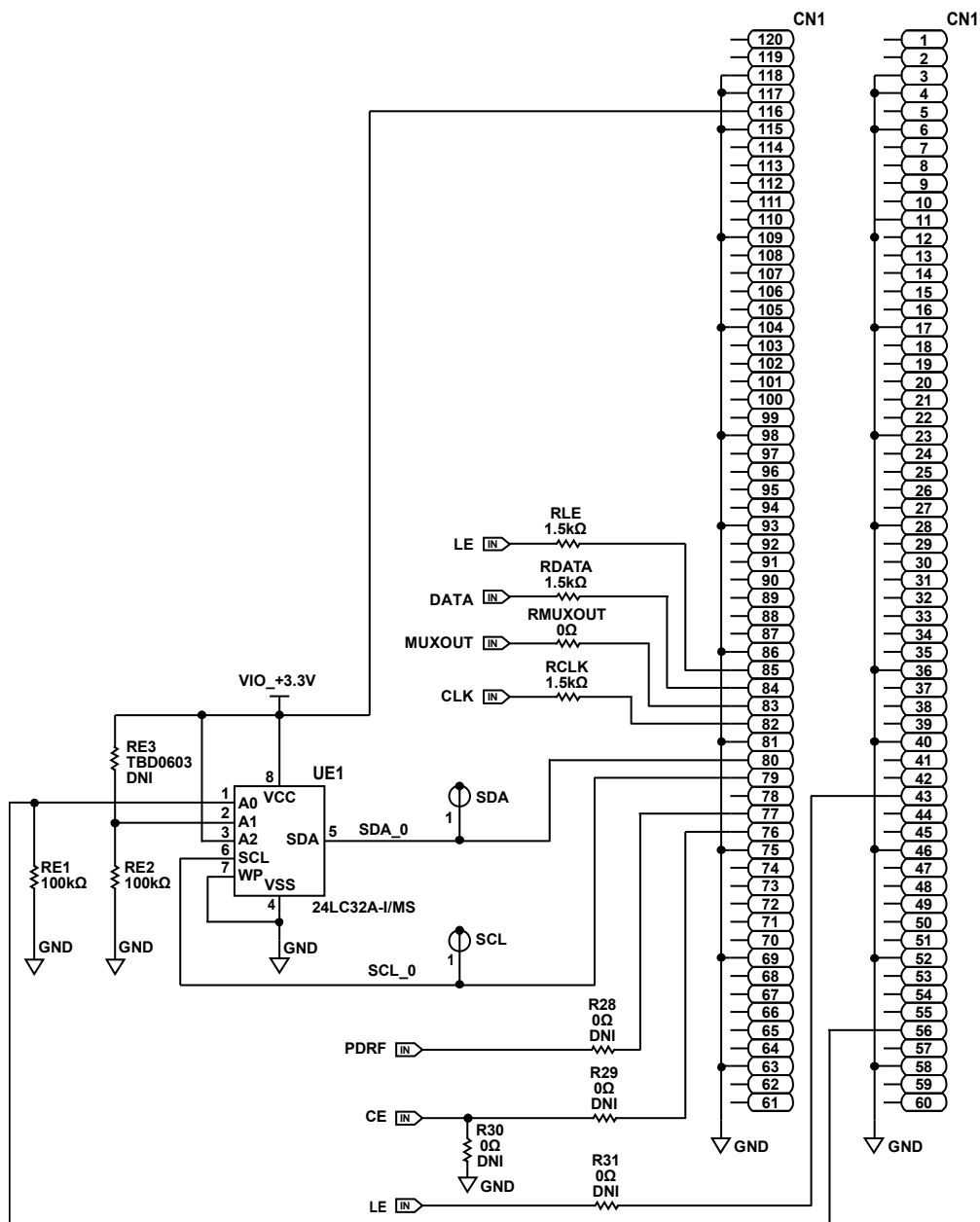
Figure 9. Evaluation Board Schematic—Page 3
