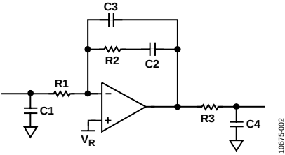
Figure 2. ADIsimPLL Filter
