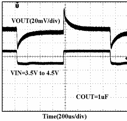
Line Transient Response (COUT=1uF)
