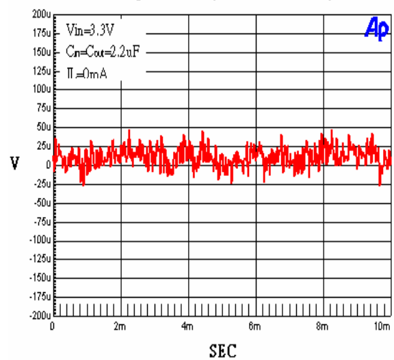
Output1 Niose(10Hz to 100KHz)
