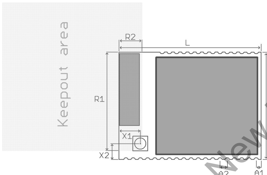
Figure 7. ETRX3 Physical Dimensions
