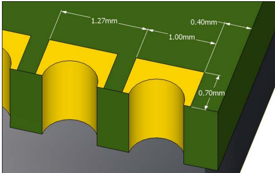
Figure 11. Typical pad dimensions
