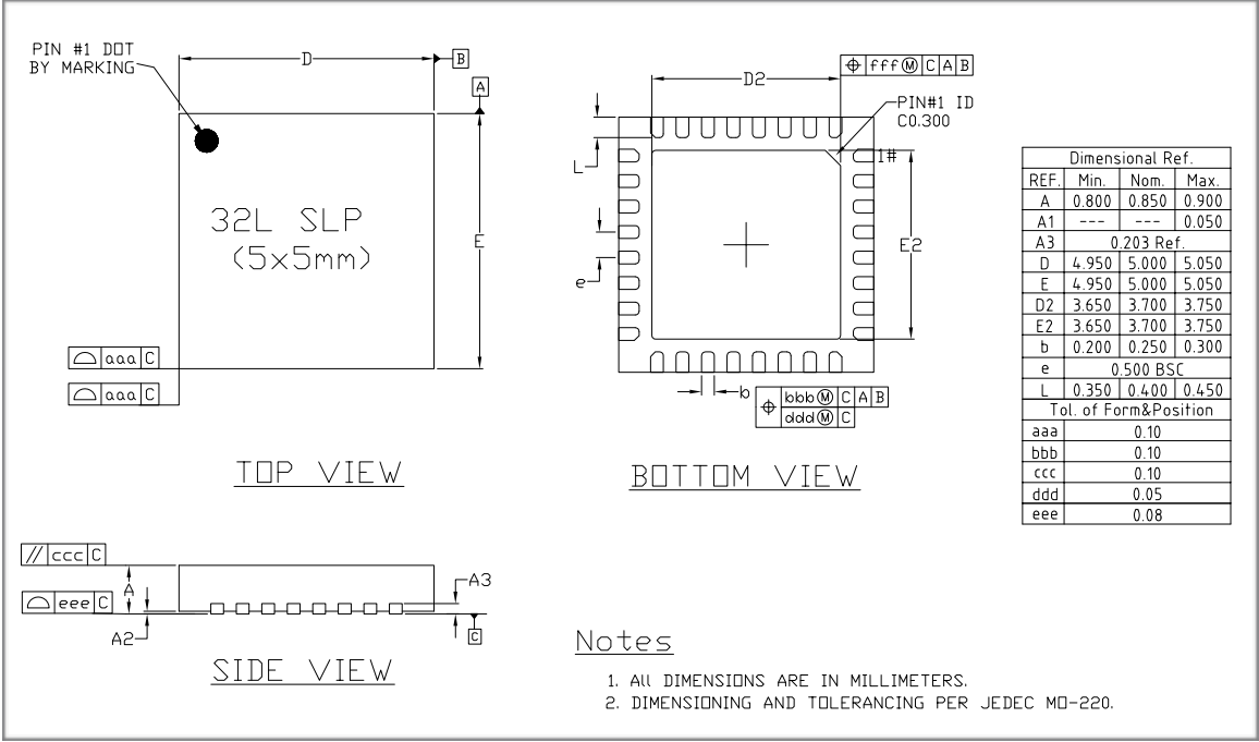
Figure 6-1. ESP8266EX Package
