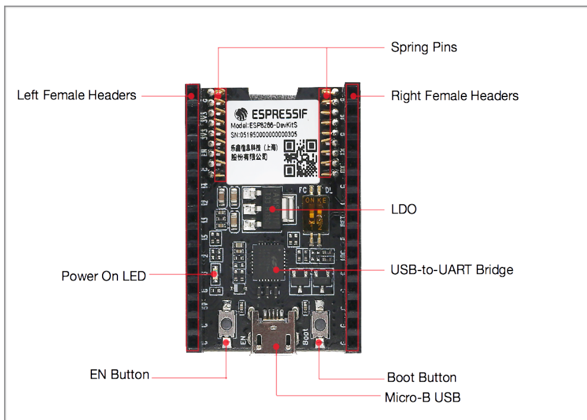
Figure 2-1. ESP8266-DevKitS
