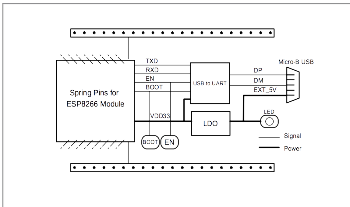
Figure 5-1. ESP8266-DevKitS Block Diagram
