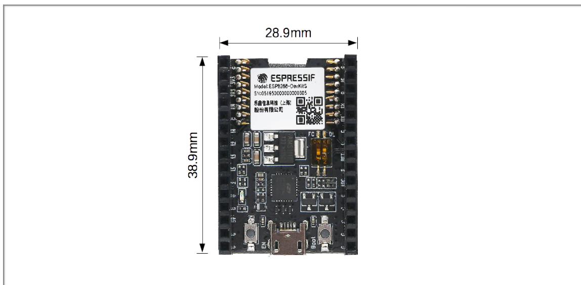
Figure 4-1. Board Dimensions
