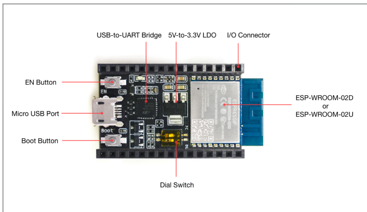
Figure 2-1. ESP8266-DevKitC
