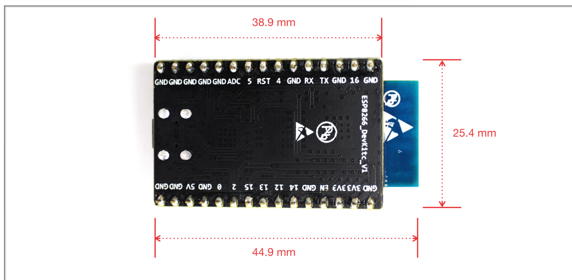
Figure 4-1. Board Dimensions
