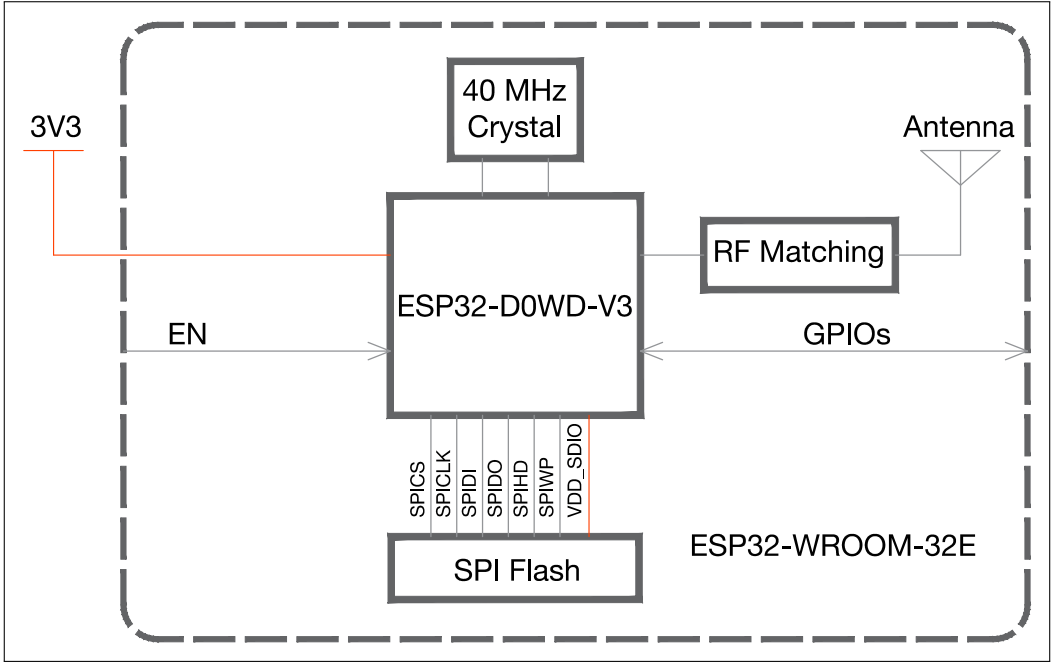
Figure 1: ESP32-WROOM-32E Block Diagram
