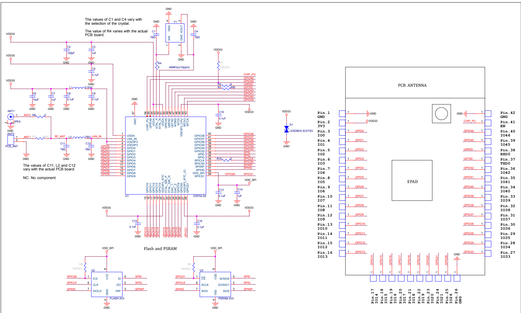
Figure 5: ESP32-S2-WROVER-I Schematics
