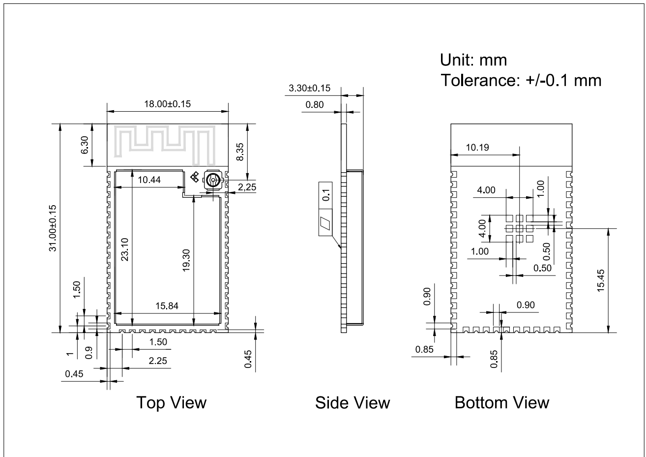
Figure 7: Physical Dimensions
