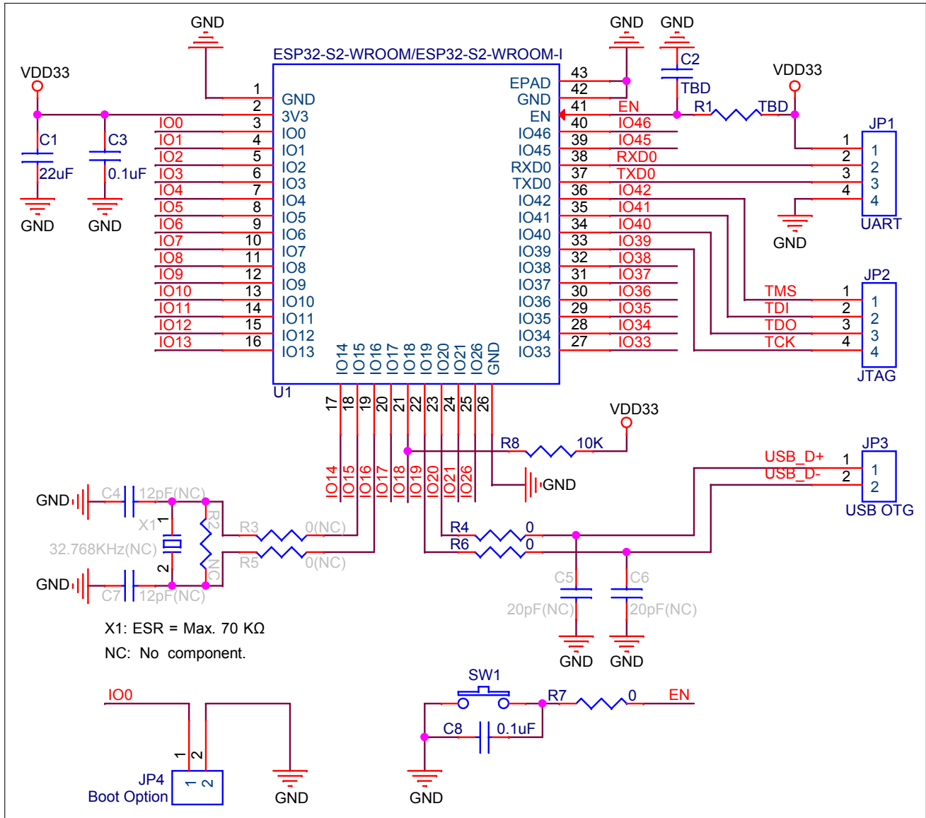
Figure 6: Peripheral Schematics
