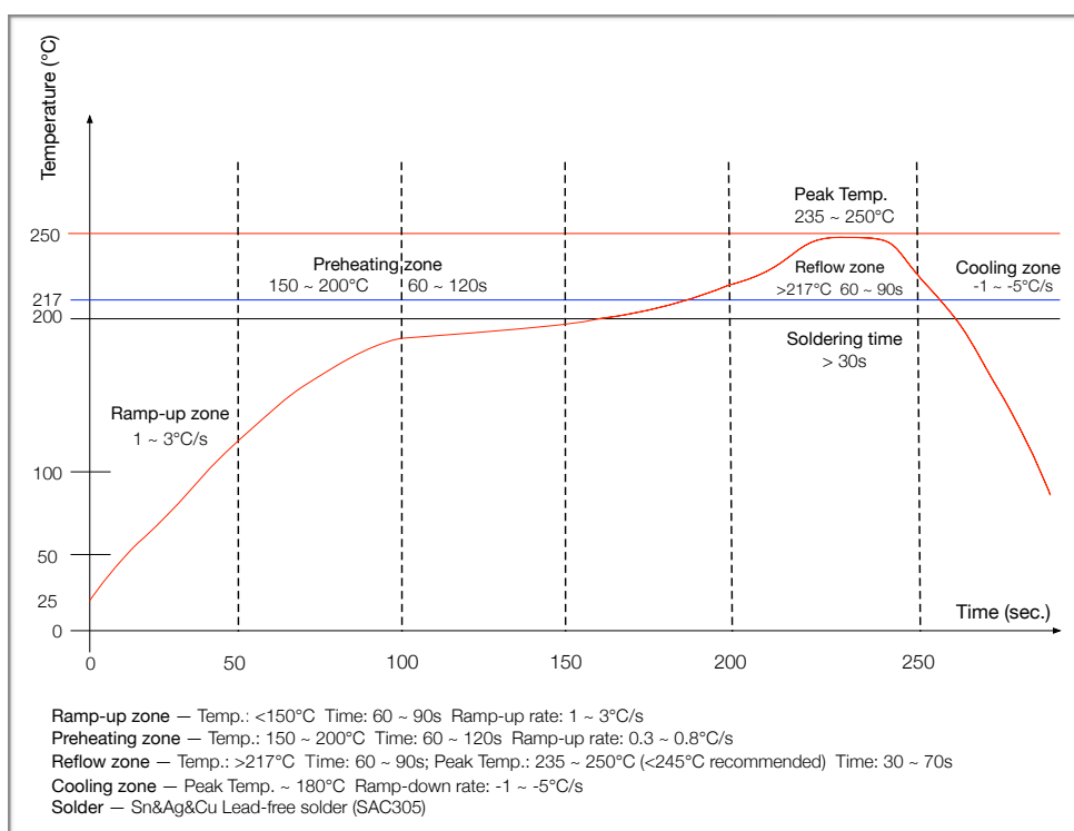
Figure 4-1. ESP-WROOM-02D/ESP-WROOM-02U Reflow Profile
