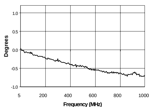
Phase Unbalance
