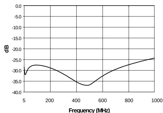
Isolation
