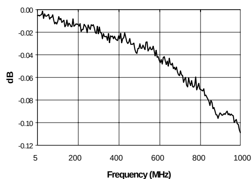
Amplitude Unbalance
