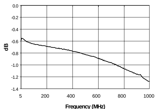
Insertion Loss
