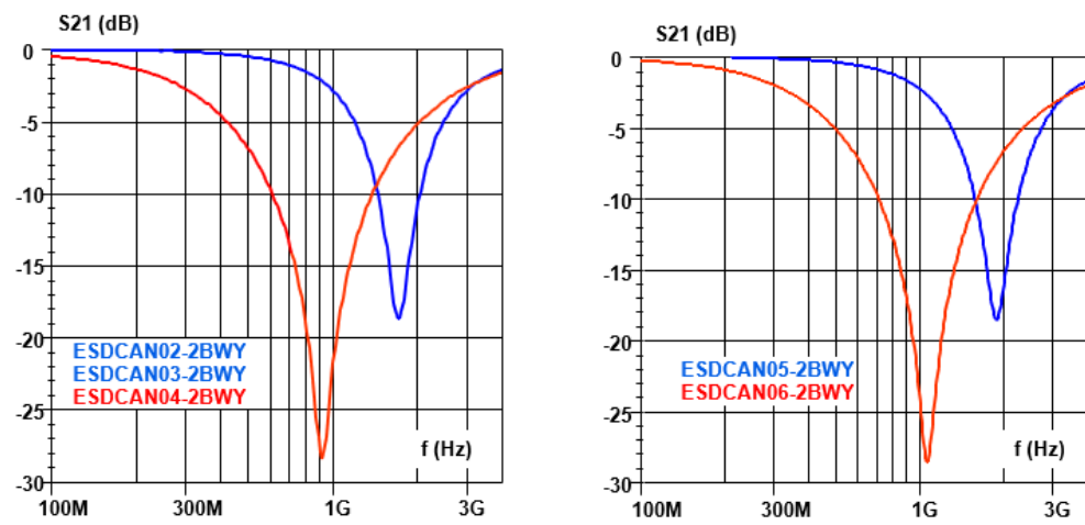
Figure 13. S21 attenuation
