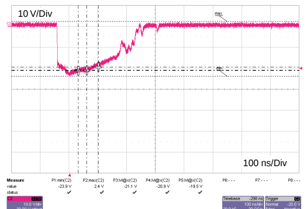
Figure 12: ESD response to IEC 61000-4-2 (-15 kV air discharge)
