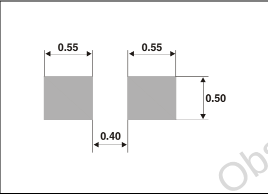
Figure 24. Footprint
