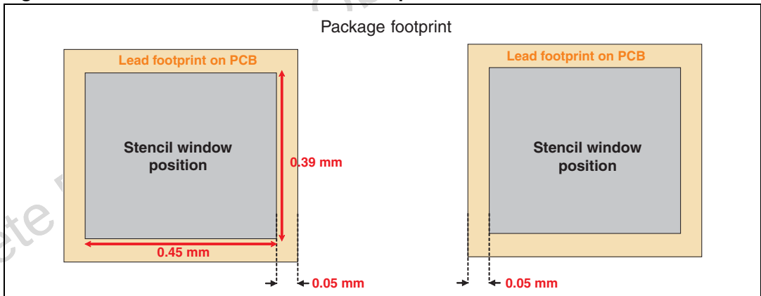
Figure 28. Recommended stencil windows position
