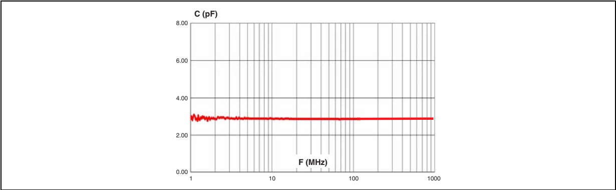
Figure 7. Junction capacitance versus frequency (typical values)
