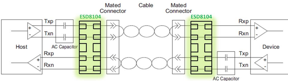
Figure 16. USB 3.0/3.1 Connection Diagram
