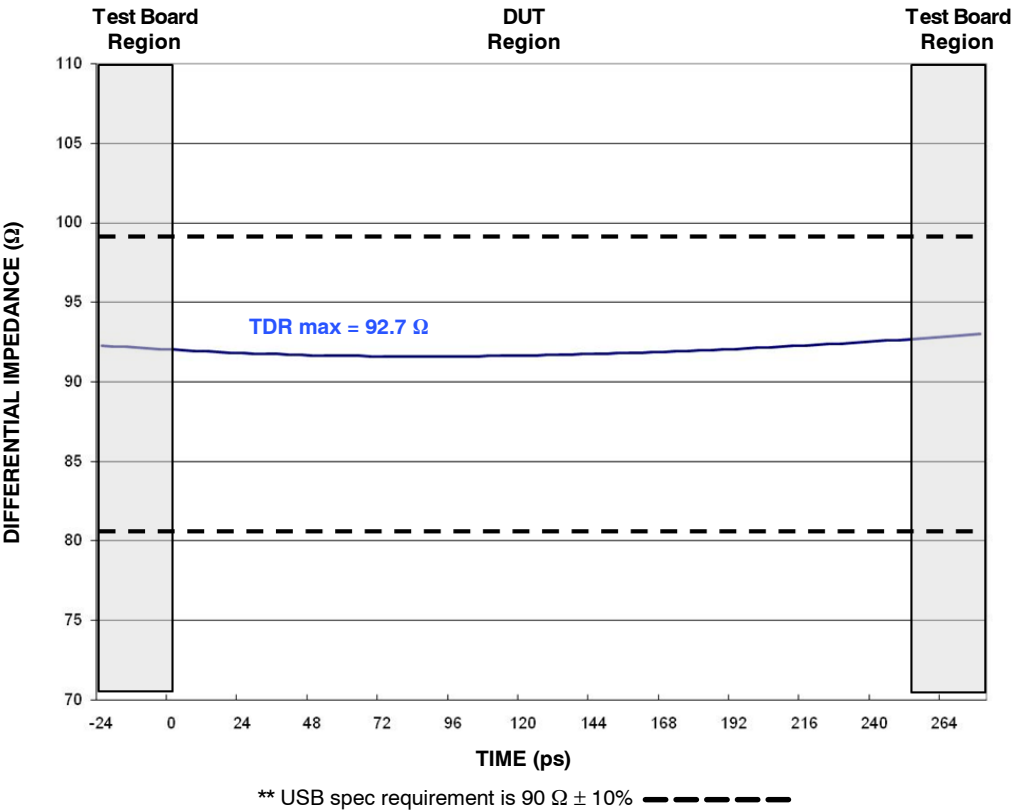
Figure 13. USB TDR Measurement. 90 \Omega Differential Impedance Target, 200 ps Rise Time
