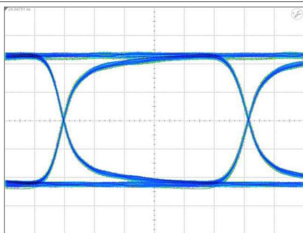
Figure 17. HDMI 2.0 6-Gbps Eye Diagram Without ESD122
