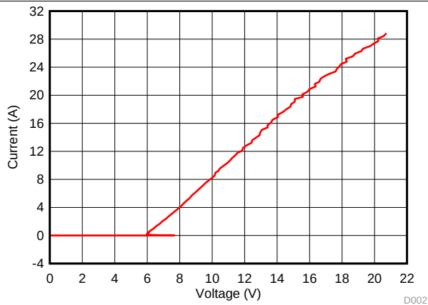
Figure 1. Positive TLP Curve, IO Pin to GND
