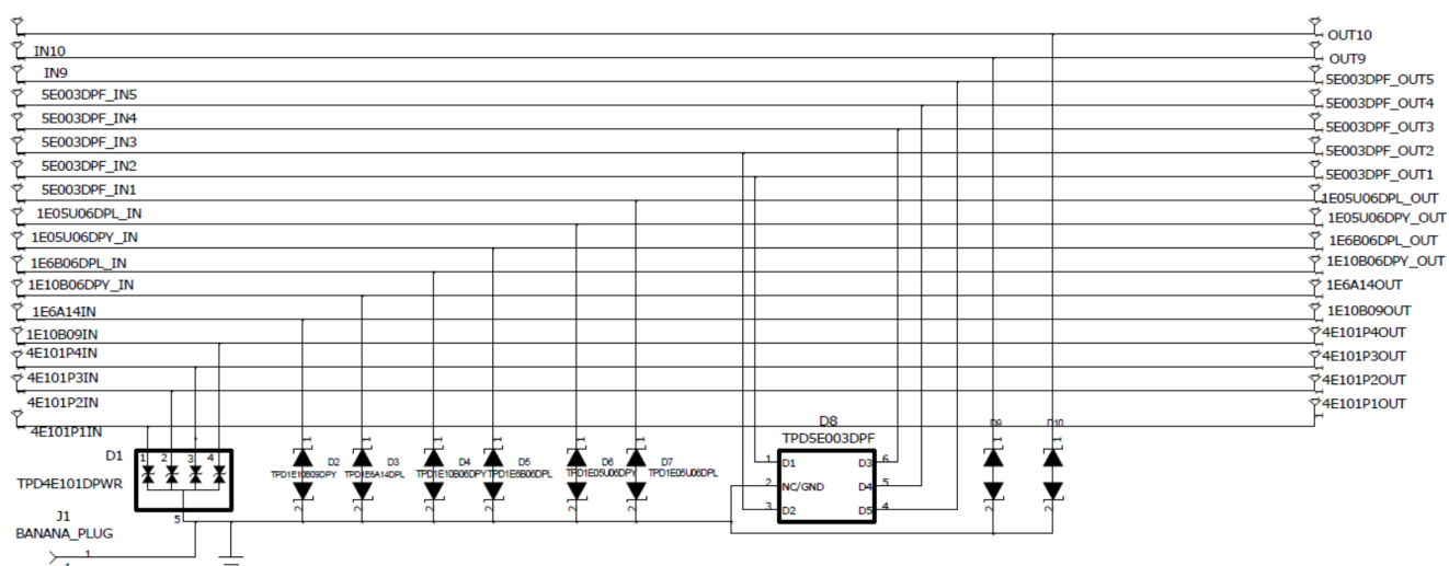
Figure 1. ESD EVM Schematic
