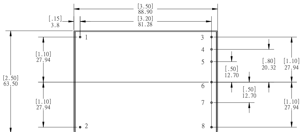
PIN - OUT VIEWED FROM BOTTOM
