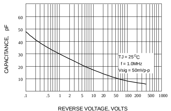
Fig. 6-TYPICAL JUNCTION CAPACITANCE
