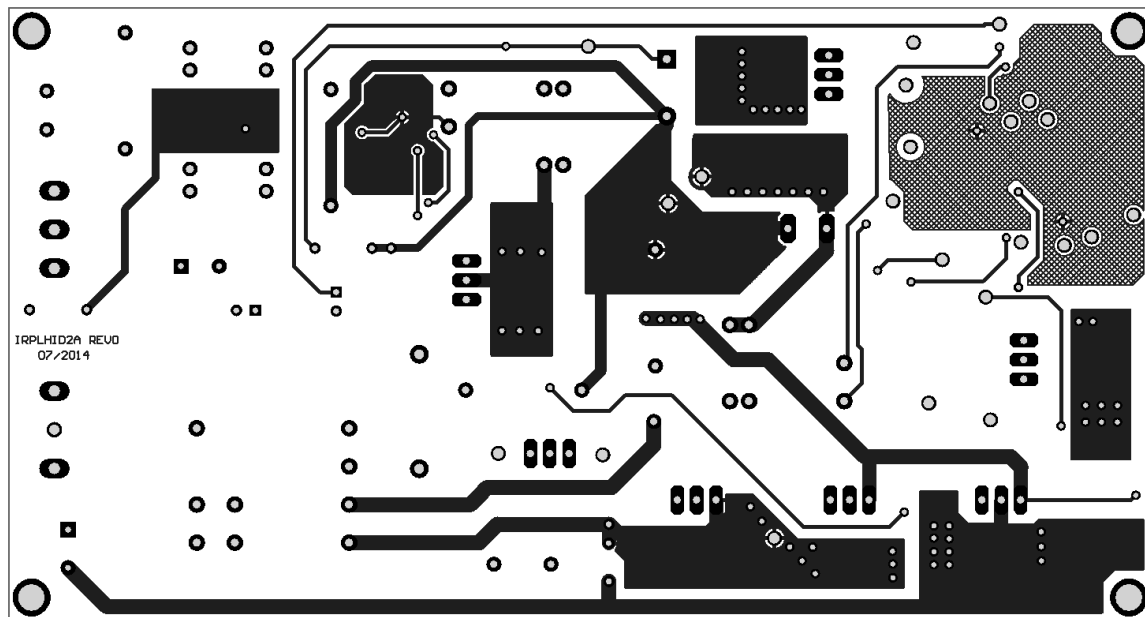
Top Copper
