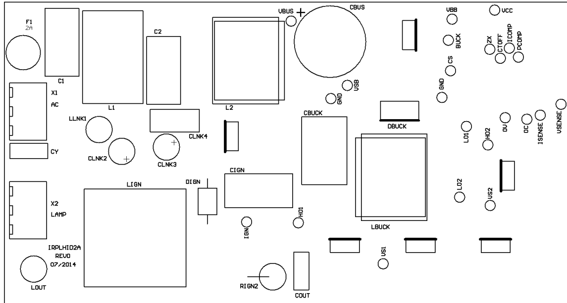
Top Assembly
