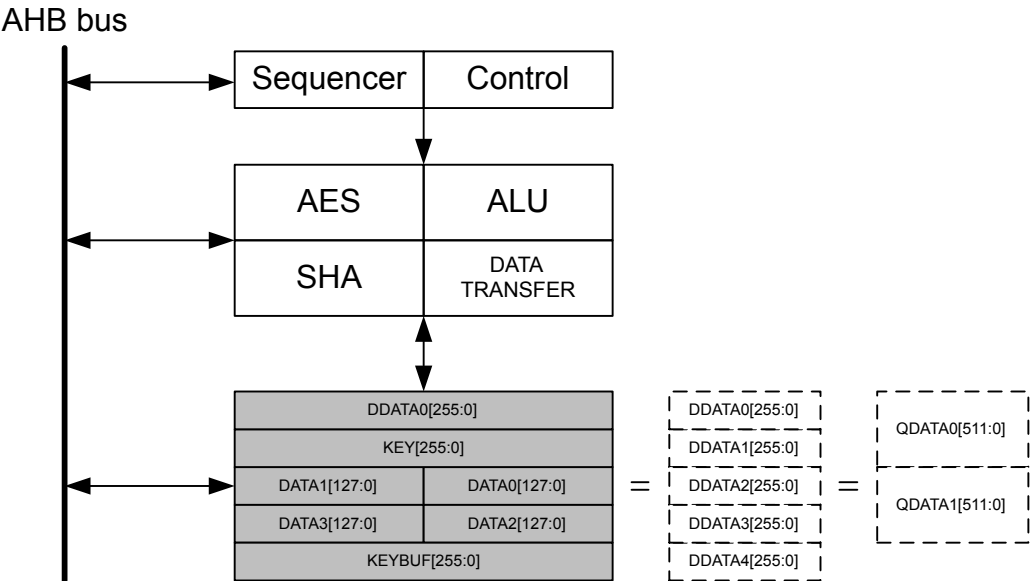
Figure 32.1. CRYPTO Overview
