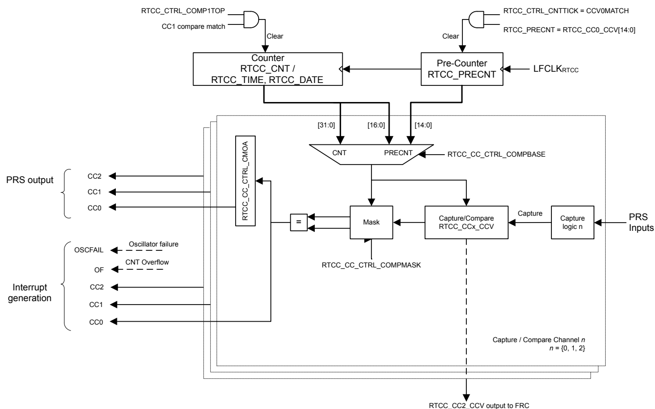
Figure 14.1. RTCC Overview
