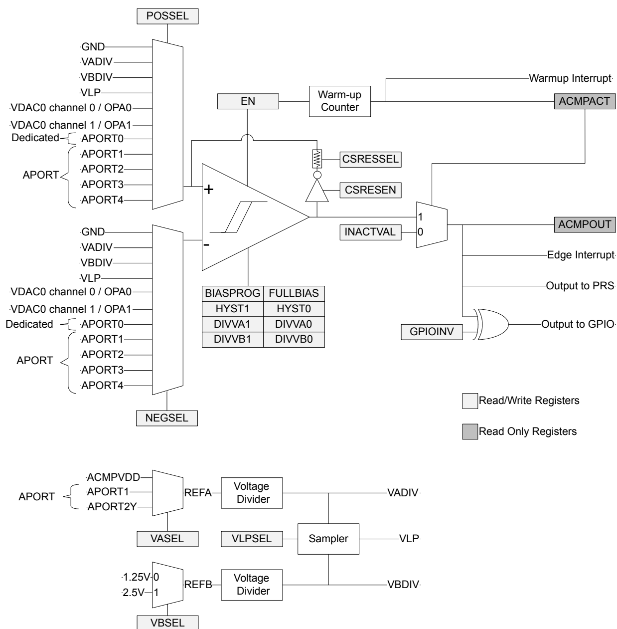
Figure 26.1. ACMP Overview
