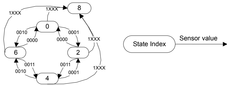
Figure 29.19. FSM Example 2
