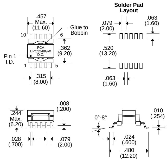
Package ER11
