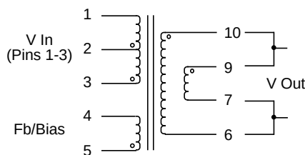
Schematic 1
