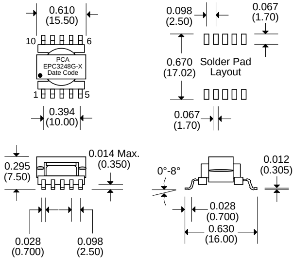
Package ER14.5
