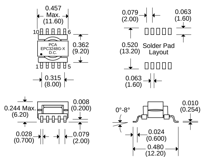
Package ER11
