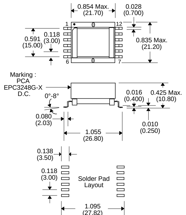
Package EFD20 (Reserved for Class 4 PoE+)
