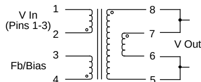
Schematic 2
