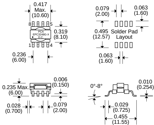
Package ER9.5
