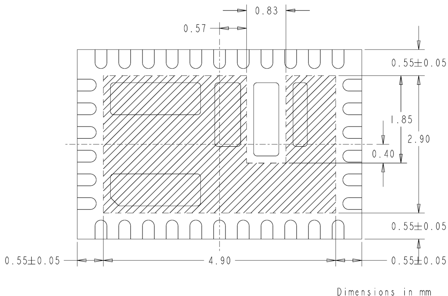
Shaded area highlights exposed metal that is not to be mechanically or electrically connected to the PCB.
