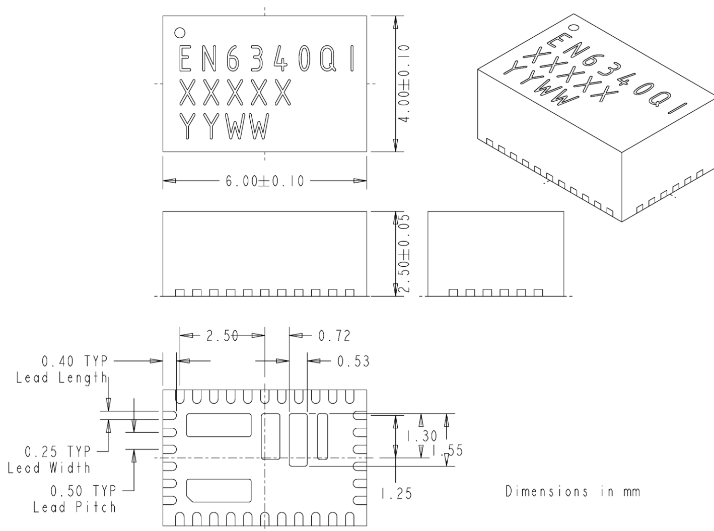
Figure 12: EN6340QI Package Dimensions
