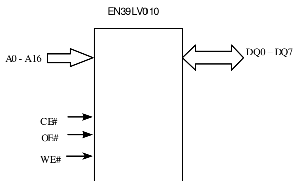
FIGURE 1. LOGIC DIAGRAM
