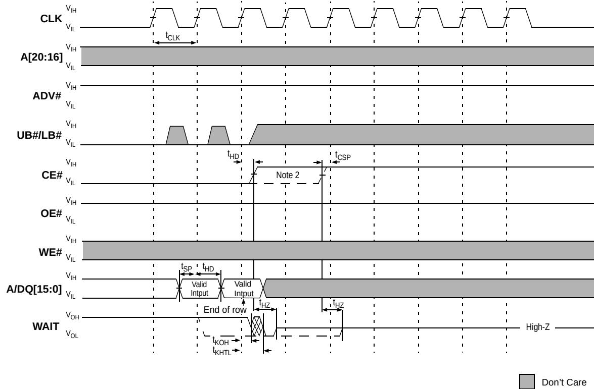
Figure 33: Burst WRITE Terminate at End-of-Row (Wrap Off)
