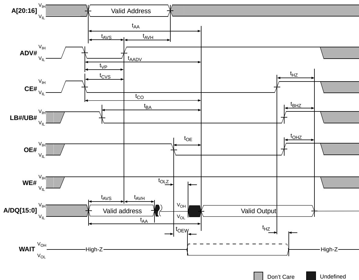
Figure 23: Asynchronous READ
