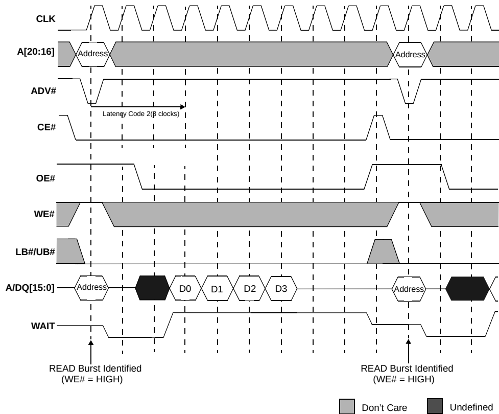
Figure 5: Burst Mode READ (4-word burst)
