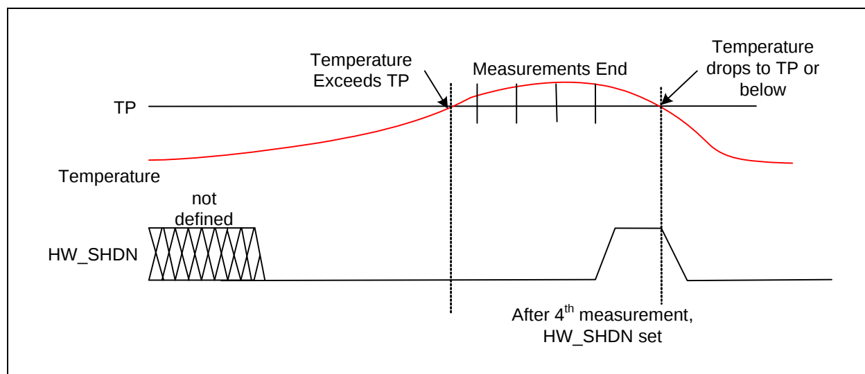
Figure 5.5 HW_SHDN Operation
