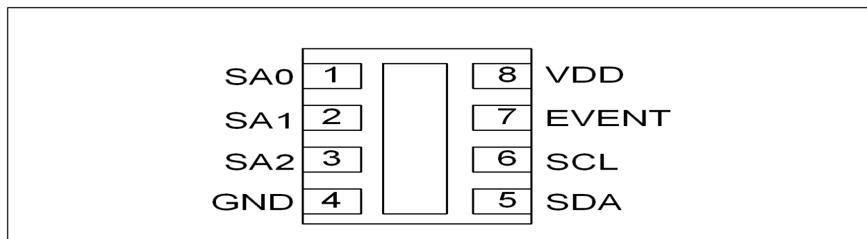
Figure 1.1 Pin Diagram
