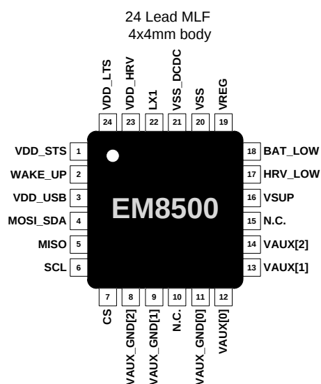
Figure 1-1 QFN24 Package
