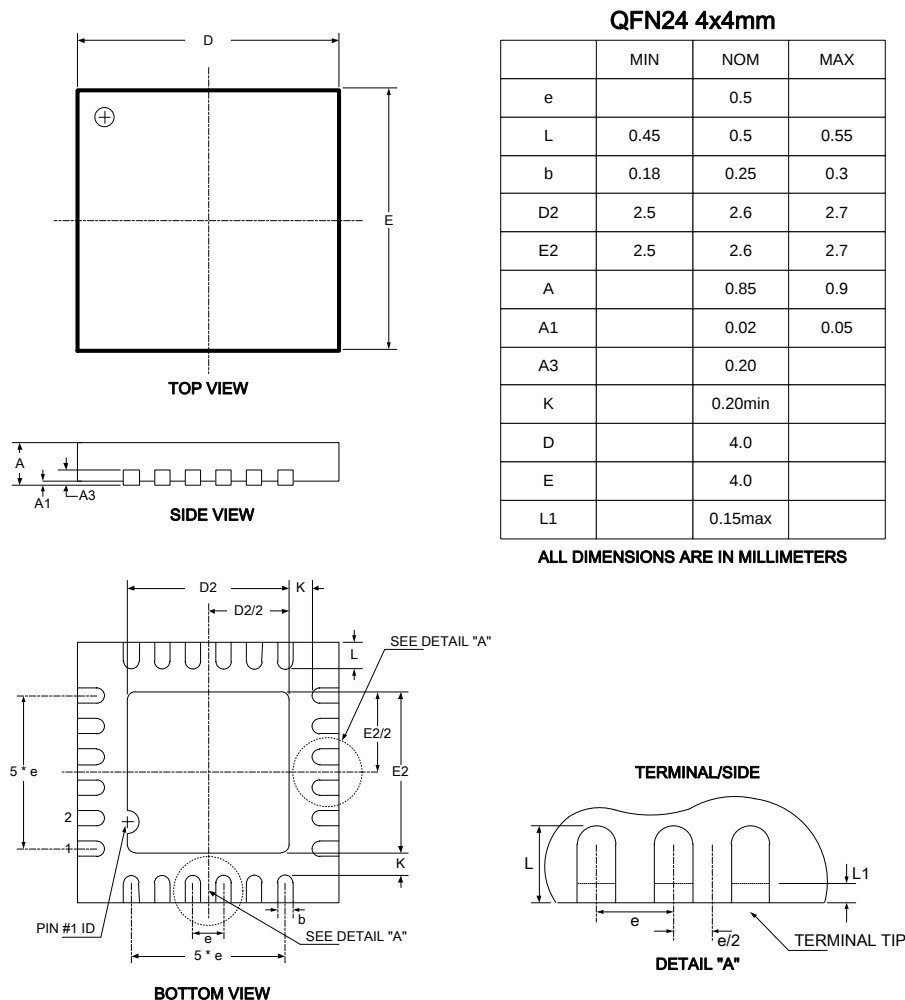
Figure 11-1 QFN24 Mechanical Information
