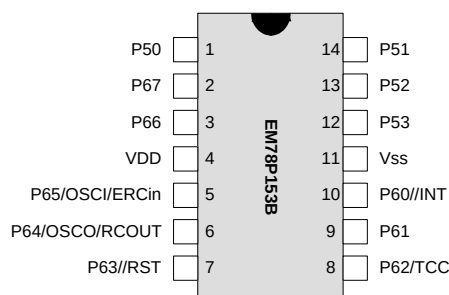
Figure 3-1a EM78P153BD14, EM78P153BSO14
