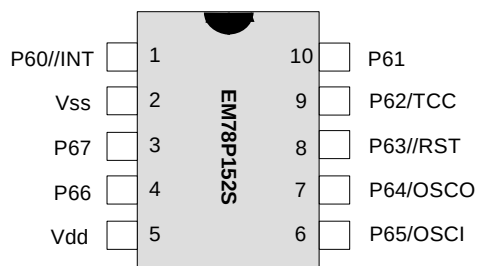
Figure 3-2 EM78P152SN/S/J
