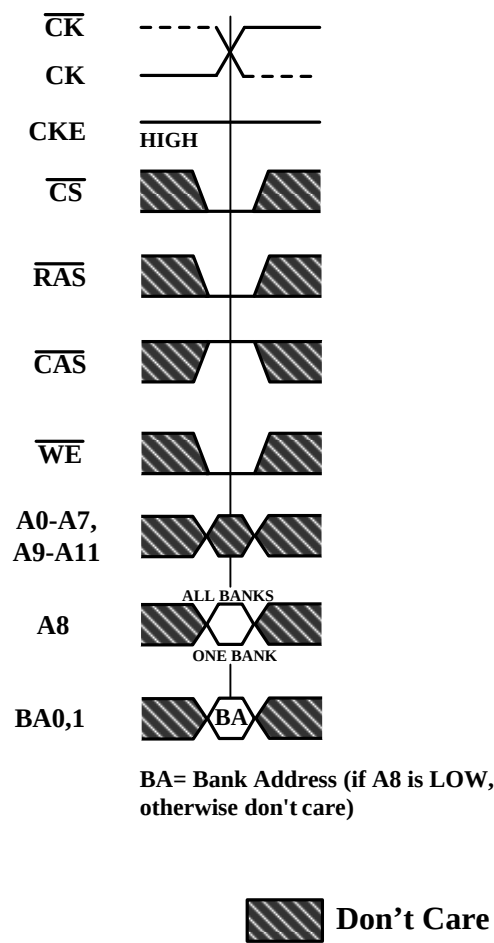
Figure 27. Precharge Command
