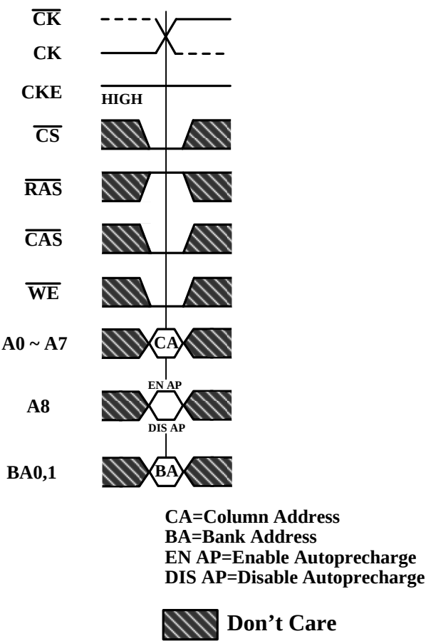
Figure 14. Write Command
