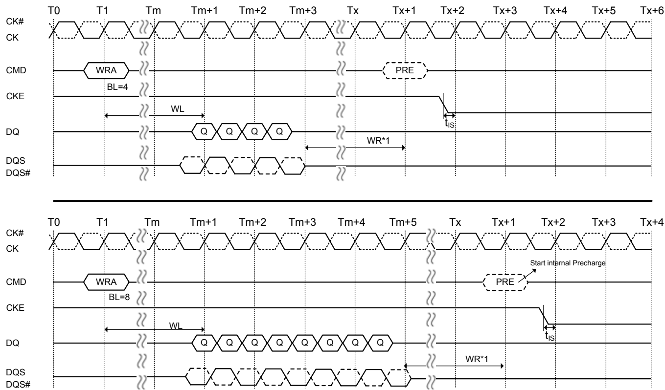
Figure 54. Write with autoprecharge to power-down entry
