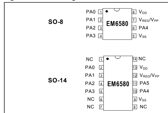
Figure 2. Pin Configuration
