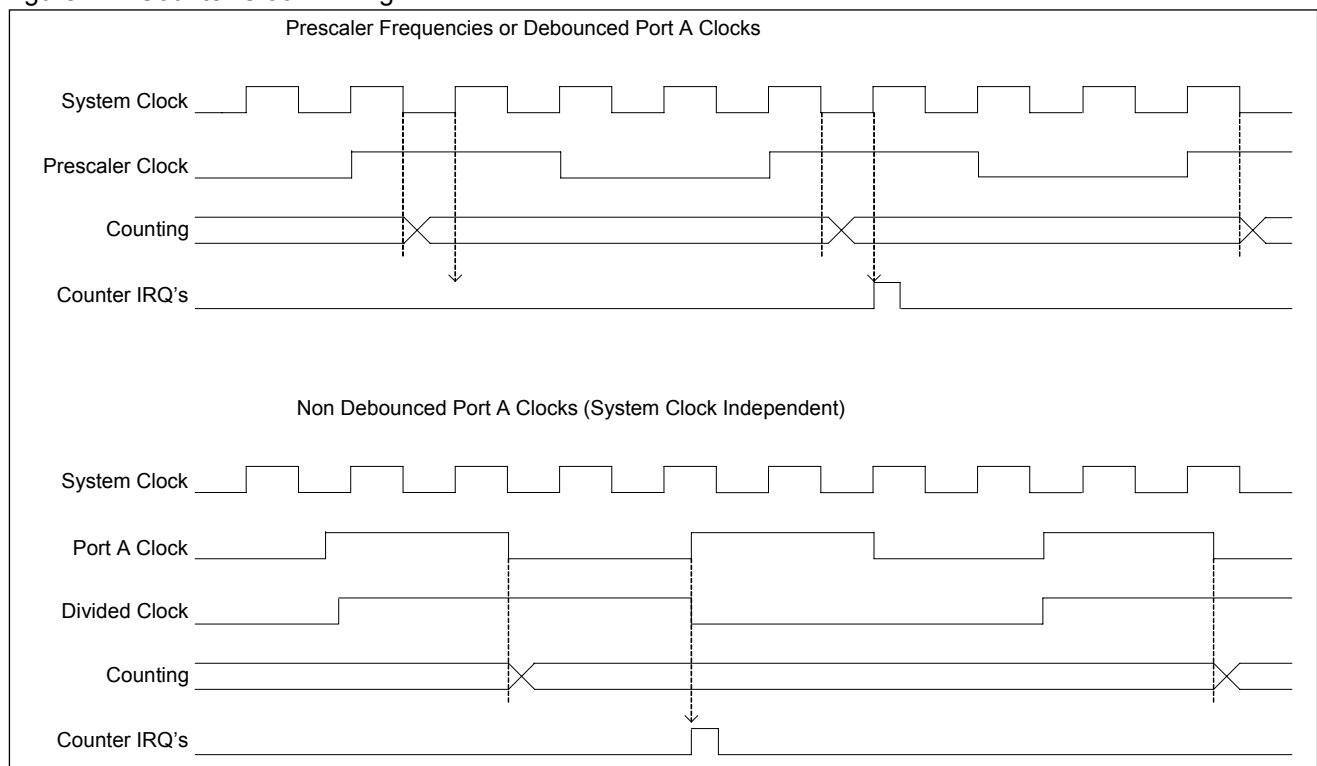
Figure 17. Counter Clock Timing
