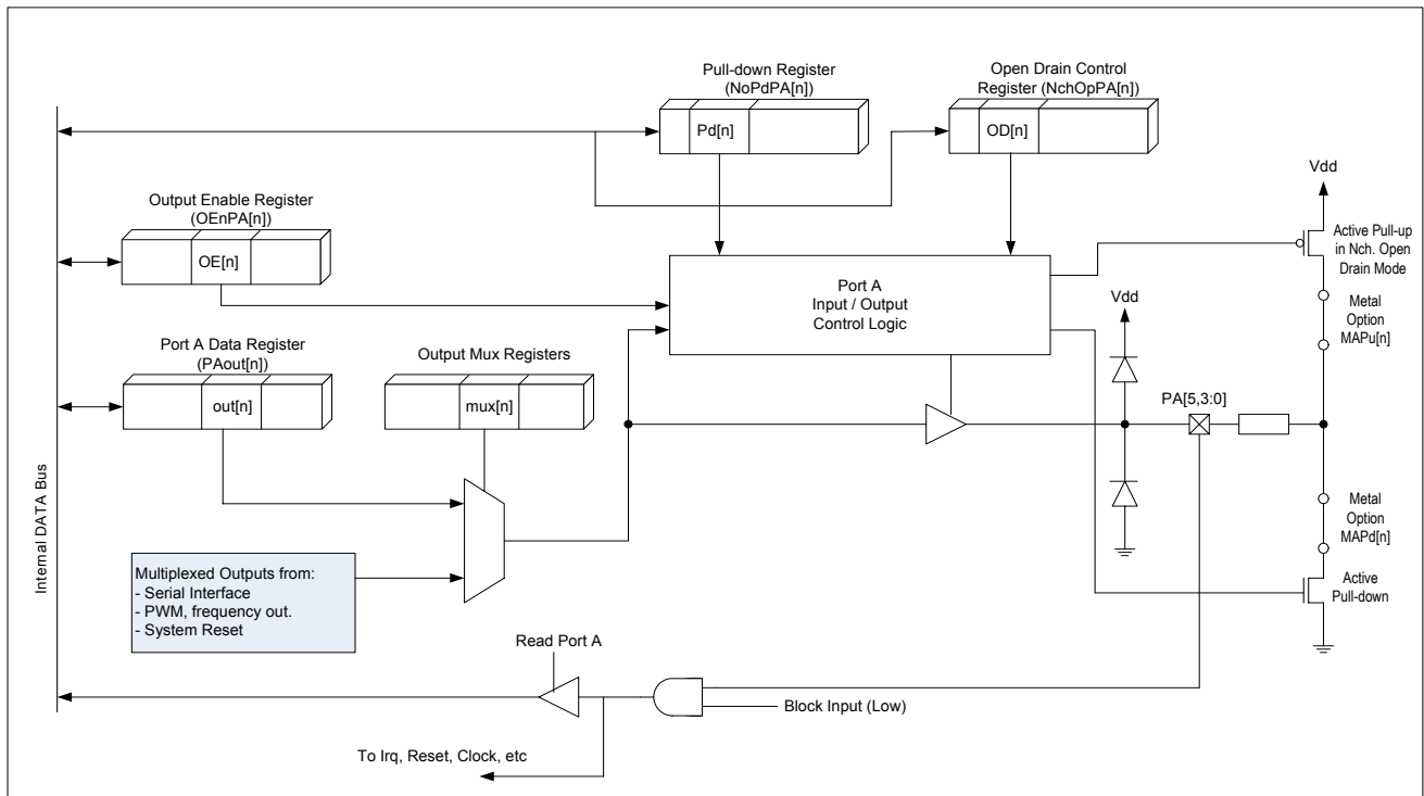
Figure 10. Port A Architecture (Outputs)
