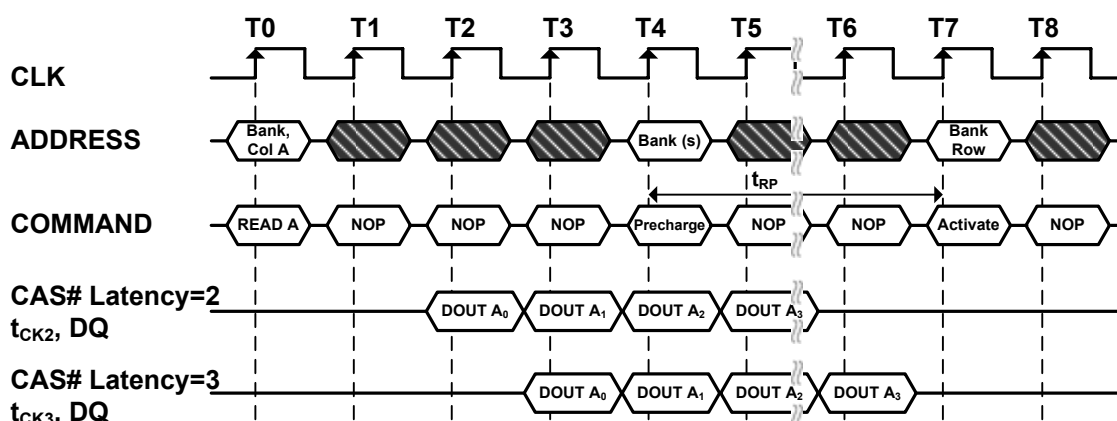
Figure 10. Read to Precharge (CAS# Latency = 2, 3)
