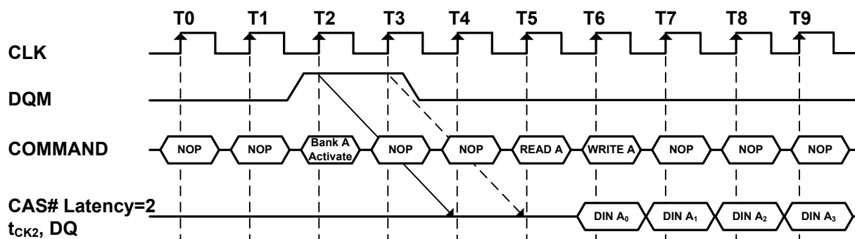
Figure 7. Read to Write Interval (Burst Length ≥ 4, CAS# Latency = 2)
