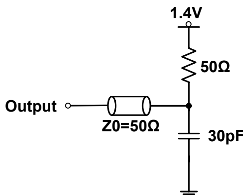
Figure 19.2 LVTTL A.C. Test Load (B)
