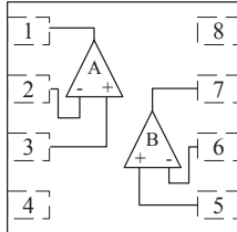
TSON8-2×2(TOP VIEW)
