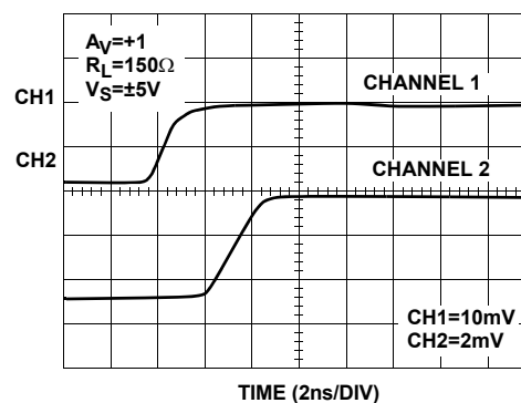
FIGURE 18. SMALL SIGNAL RISE TIME
