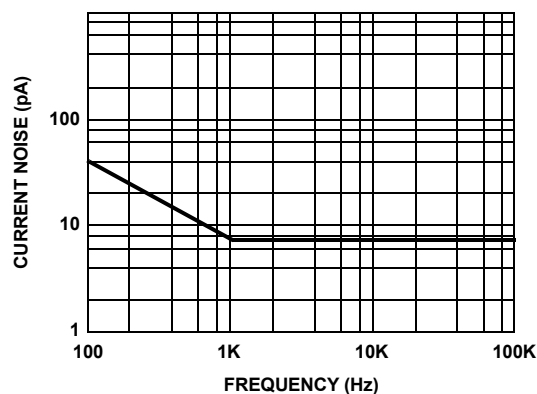
FIGURE 20. CURRENT NOISE
