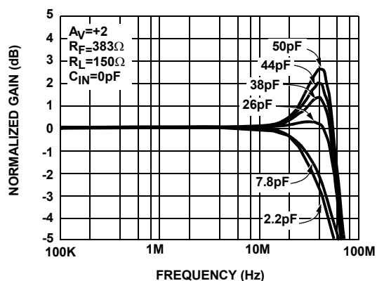
FIGURE 24. GAIN vs FREQUENCY FOR VARIOUS C_L
