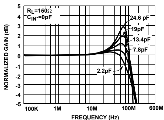
FIGURE 22. GAIN vs FREQUENCY FOR VARIOUS C_L
