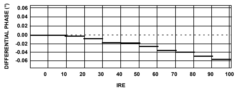
FIGURE 28. DIFFERENTIAL PHASE (°)
