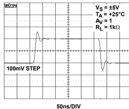
FIGURE 26. SMALL SIGNAL TRANSIENT RESPONSE
