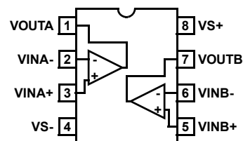
EL5211A (8 LD HMSOP) TOP VIEW
