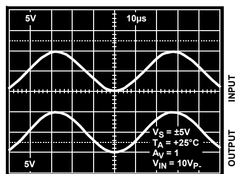
FIGURE 27. OPERATION WITH RAIL-TO-RAIL INPUT AND OUTPUT
