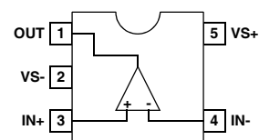
EL5192 (5 LD SOT-23) TOP VIEW
