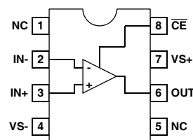
EL5192A (8 LD SOIC) TOP VIEW
