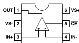
EL5192A (6 LD SOT-23) TOP VIEW
