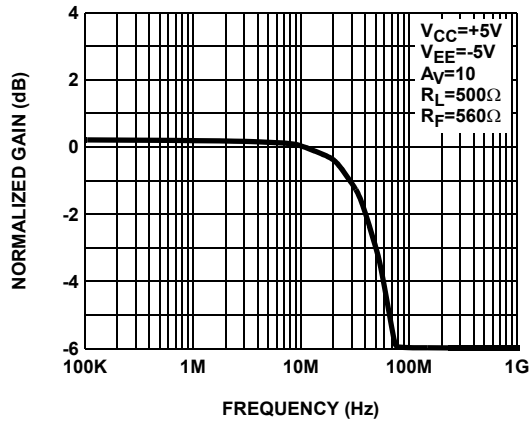
FIGURE 5. FREQUENCY RESPONSE
