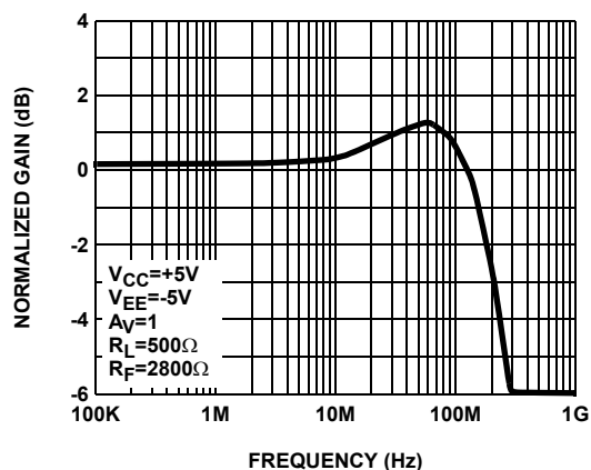
FIGURE 2. FREQUENCY RESPONSE
